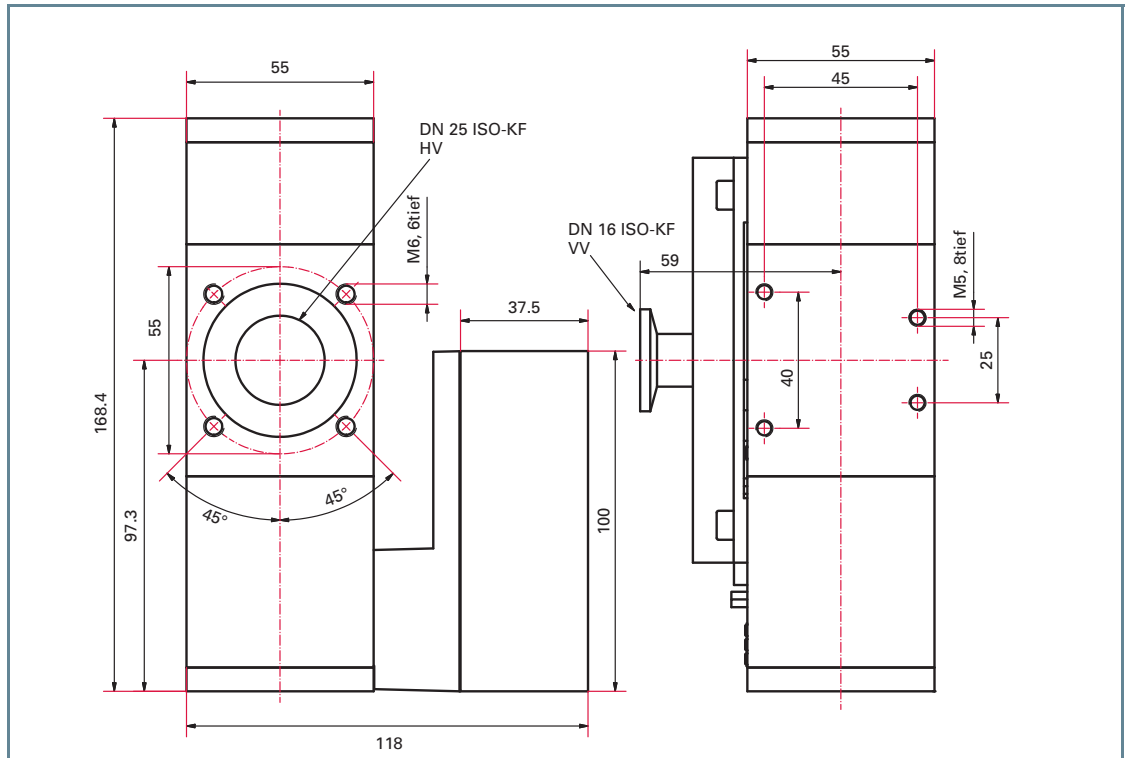
HiPace™ 10, with TC 110, DN 25
